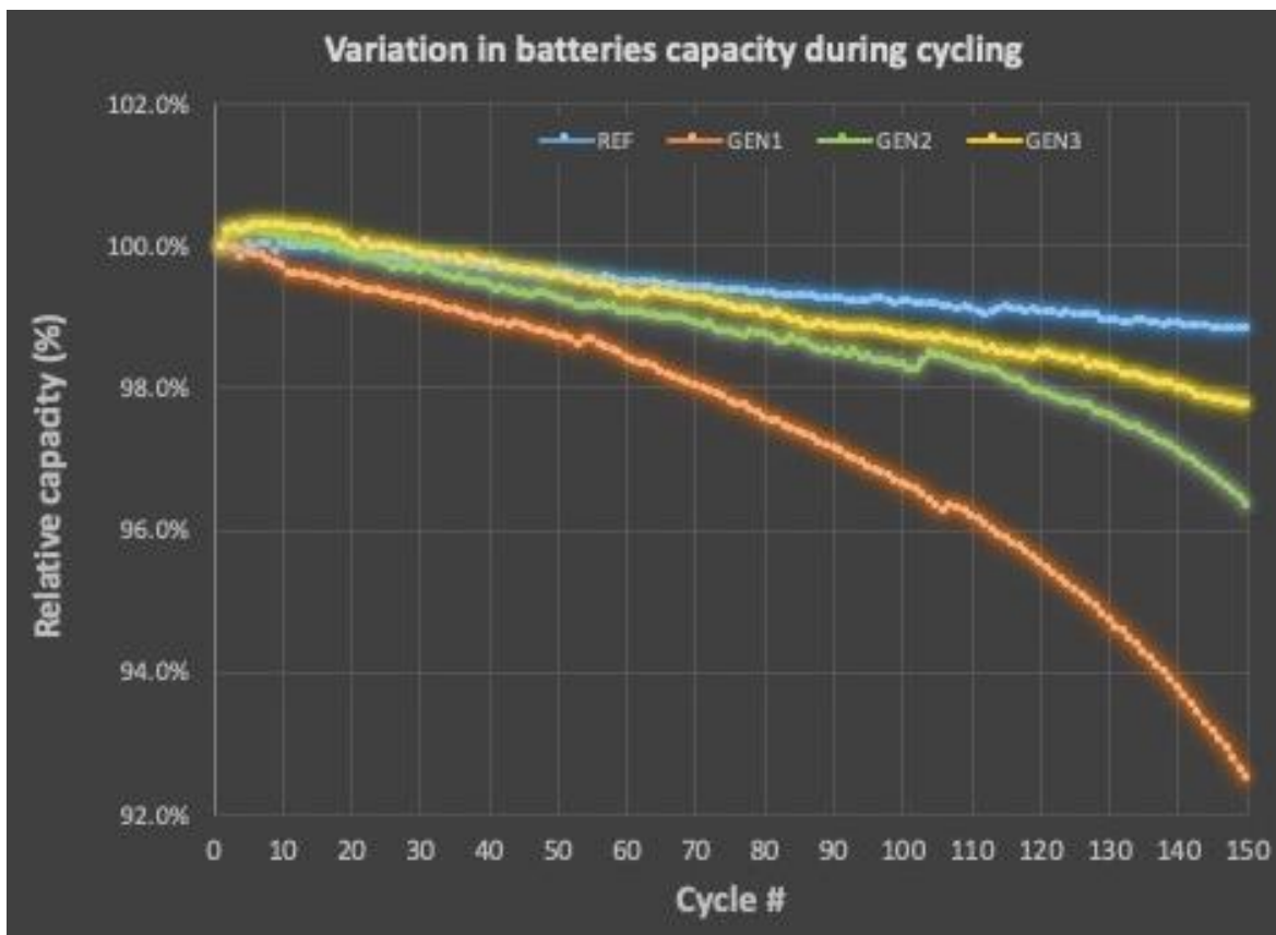
Graph 2) the blue line shows the relative capacity of 100% graphite batteries, the orange line the relative capacity of GEN1 batteries, the green line the relative capacity of GEN 2 batteries and the yellow line shows the relative capacity of GEN 3 batteries over 150 cycles [1]
