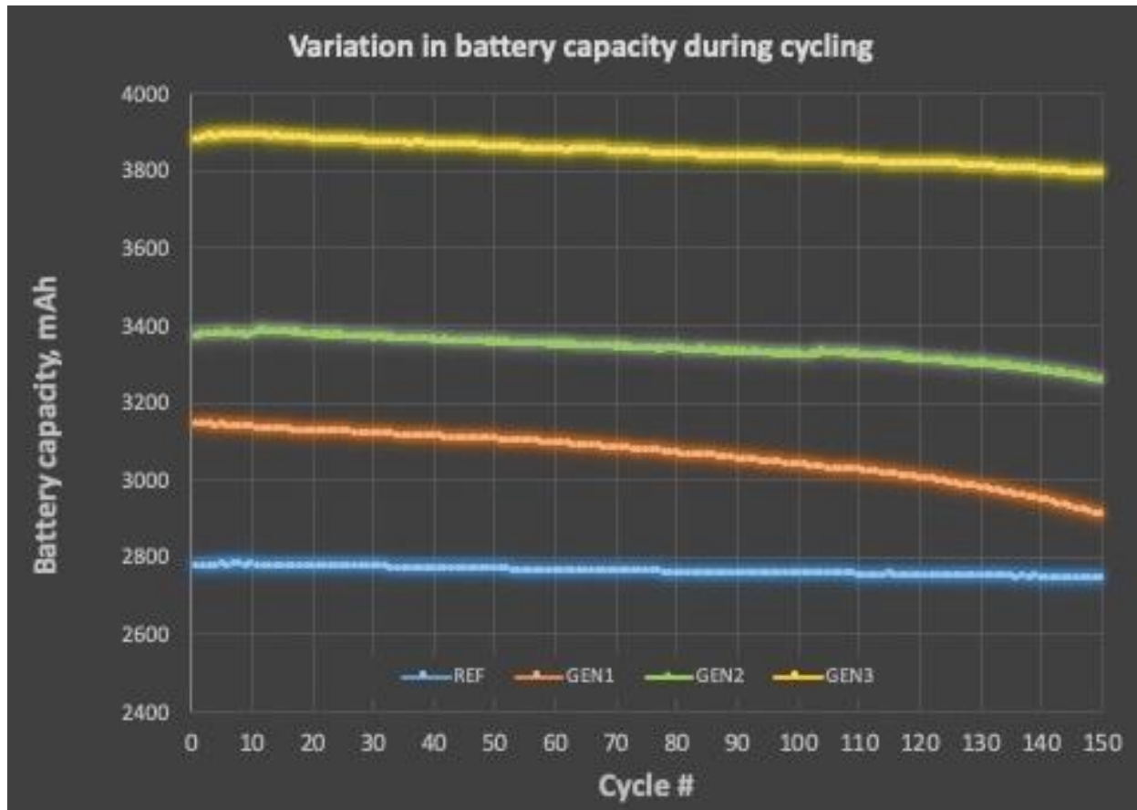
Graph 1) Average capacity, in milliampere-hours (mAh), of 100% graphite, GEN1, GEN2 & GEN3 batteries over 150 cycle testing [1] (the blue, orange, green and yellow lines).
